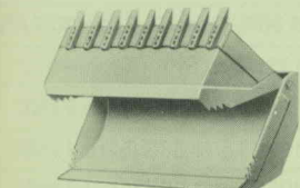
MULTIPURPOSE BUCKET A bucket/blade combination usable as a bucket, blade, scraper or clamshell for all-around loading, topsoil stripping and debris cleaning.
