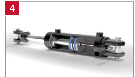
Internally mounted sensing technology: Precise control and feedback.
