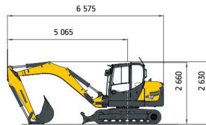
Fig. 2: Position de transport
