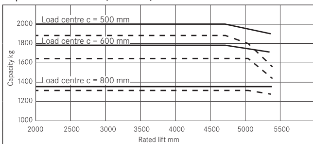
Capacities RX 20-20P/h Tele -/ HiLo - mast
