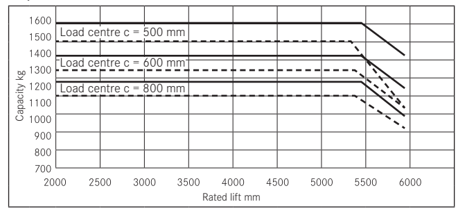
Capacities RX 20-16 Tele -/ HiLo - mast
