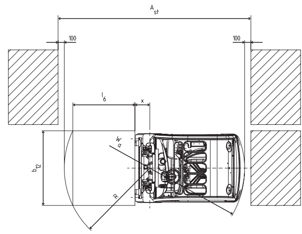
Dimensions relate to a vertical mast
