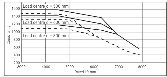
Capacities RX 20-16 Triplex mast
