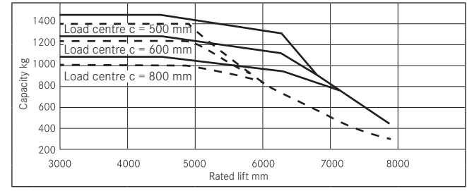
Capacities RX 20-15 Triplex mast
